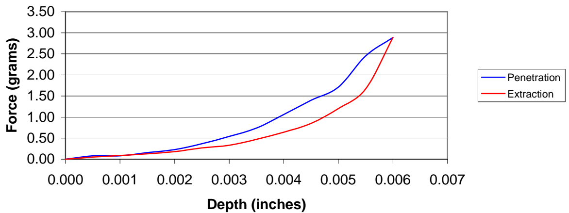
Probe Form 15003SCM / 1.0 mil Flat Tip
