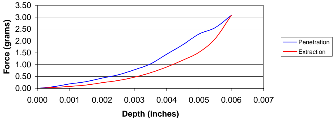
Probe Form 15003SCM / 1.5 mil Flat Tip
